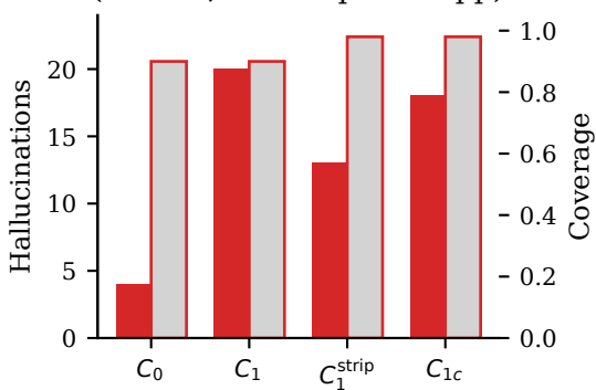
Mode B: training-prior leak (Claude, Heat Pipes 104pp)
