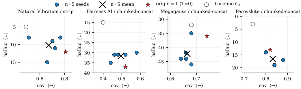
Figure 7: n = 5 multi-seed envelopes for the four intervention-verification cells. Blue dots are the five Pass-2 seeds at T = 0.7 ; the black \times is the n = 5 mean; the red star is the originally-published n = 1 point at T = 0 ; the open circle is the cell’s C_1 baseline (no intervention). On NV strip, Fairness AI, and Perovskite the original n = 1 value sits within the n = 5 envelope; on Megagauss the original is outside the envelope on both axes (lower halluc and higher cov than any of 5 seeds), and the mean C_{1c}^{\text{concat}} effect on coverage is essentially zero — so the published Megagauss chunked-Pass-2 cov-gain claim is retracted at n = 5 .
