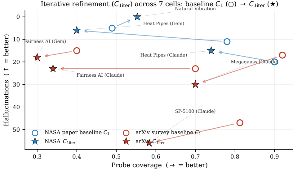
Figure 9: Iterative-refinement Pareto frontier across 7 cells. Each cell’s baseline C_1 (open circle) is connected by an arrow to its C_{1iter} result (filled star). Blue cells are NASA papers; red cells are modern arXiv surveys. NASA papers (Natural Vibration, Heat Pipes both vendors) move up-left: hallucinations down, coverage either up (Natural Vibration, Pareto-positive) or down (Heat Pipes, trade). arXiv surveys (Fairness AI, SP-5100, Megagauss) move down-left: both axes worse, because the Pass-2b rewrite step cannot fit the source’s content into the output budget once claims have been atomized.
