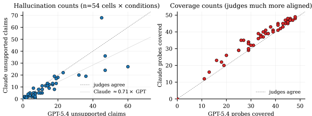
Figure 10: Inter-judge agreement on hallucinations and coverage across all cell-condition pairs. Dashed line: judges-agree identity ( y = x ). Dotted: \text{Claude} \approx 0.71 \times \text{GPT-5.4} (the median per-pair ratio). Hallucination counts (left) show Claude systematically reporting fewer unsupported claims than GPT-5.4, with most pairs falling along the 0.71 \times line; the two large outliers (top-left of left panel) are the SP-5100 and Megagauss high-count cells. Probe-coverage counts (right) are much more aligned — nearly every point sits within a few probes of the identity line — consistent with our per-probe agreement median of 0.94.
