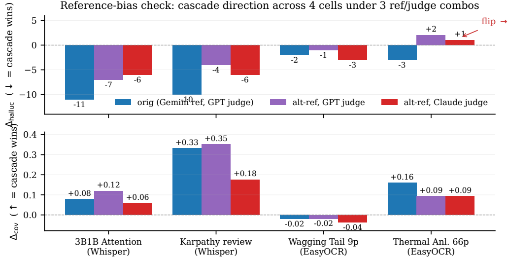
Figure 12: Reference-bias check on 4 cells (revised from 2 in the previous version). For each cell we replace the Gemini reference with a non-Gemini one (Whisper-base ASR on 3B1B Attention and Karpathy; EasyOCR on Wagging Tail and Thermal Analysis), re-extract probes with Claude, and re-judge with both GPT-5.4 and Claude. Cascade coverage direction is preserved on all four cells under both judges. Cascade hallucination direction is preserved on 3/4 cells; the exception is Thermal Analysis 66pp under EasyOCR, where the noisier OCR reference flips the hallucination axis on both judges (cascade looks +1 to +2 hallucinations rather than -3) — a reference-side bias rather than a model-side finding.
