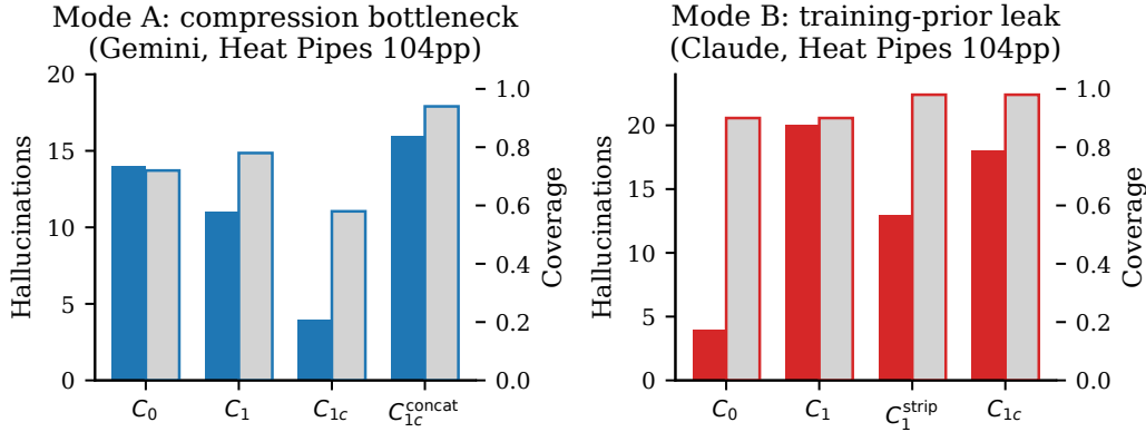
Figure 6: Two cascade failure modes on Heat Pipes 104pp. Left: Mode A (Gemini) — Pass-2 must compress 22k→1.8k words; chunked Pass-2 ( C_{1c}^{\text{concat}} ) relieves the bottleneck and lifts coverage from 0.78 to 0.94 at a +5-hallucination cost (11→16), a Pareto move along the frontier rather than strictly above it. Right: Mode B (Claude) — C_1 hallucinates 5× more than C_0 ; replacing citation surface forms (Reference N) with neutral placeholders ( C_1^{\text{strip}} ) reduces hallucinations 20→13. Hallucinations on left axis (lower better); coverage on right axis (higher better).
