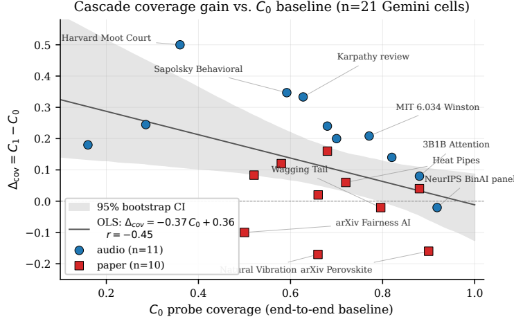
Figure 2: Cascade coverage gain vs C_0 baseline across all 21 Gemini cells. Each point is one cell; circles are audio, squares are paper. The OLS line is annotated with Pearson r = -0.45 ; the gray band is a percentile bootstrap 95% CI on the regression line. Bootstrap CI on the correlation itself: r \in [-0.73, -0.10] with fraction r \geq 0 equal to 0.9%. The five clearest counter-cells (NeurIPS panel, Natural Vibration, Wagging Tail, arXiv Fairness AI, arXiv Perovskite) sit at high C_0 baseline (no headroom) or trigger Mode A/B (§3.4).
