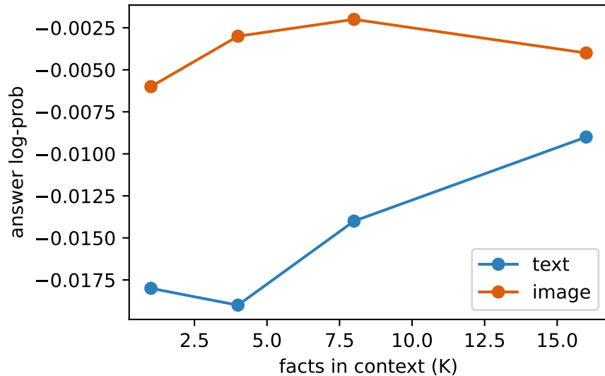
answer confidence under load
