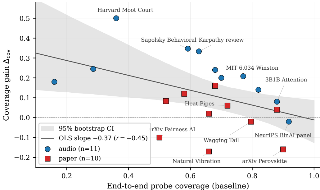
Coverage gain vs. end-to-end baseline (n=21 Gemini cells)
