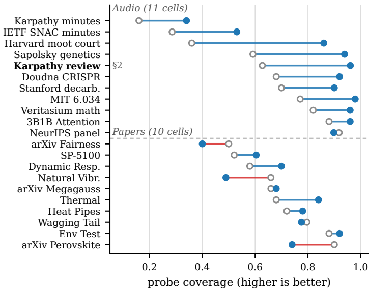
(a) Coverage, all 21 Gemini 3.1 Pro cells
