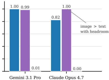
Frontier reasoning: multi-hop (sum of 6 facts)
