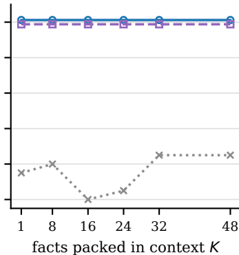
Frontier retrieval: Claude Opus 4.7
