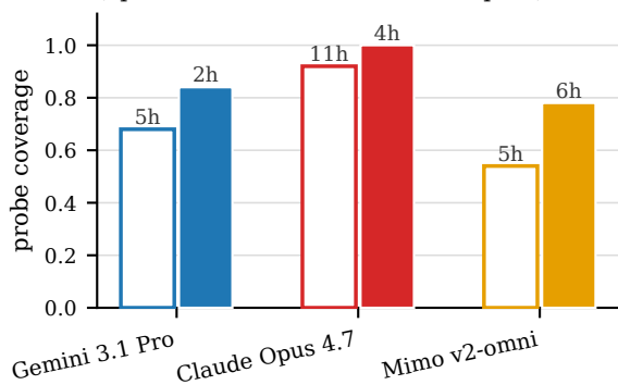
(a) Thermal: every vendor improves (open = end-to-end, filled = two-pass)
