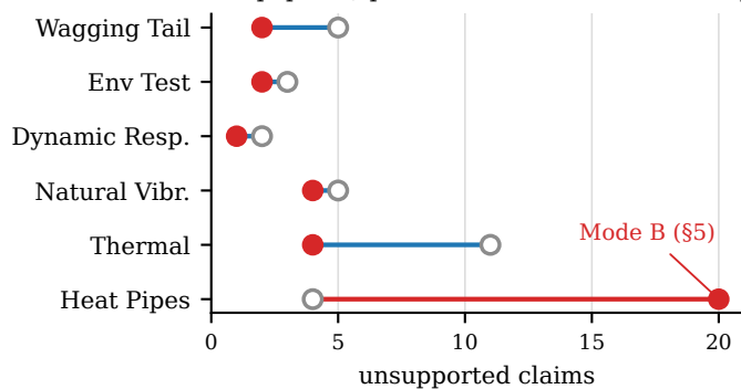
(b) Within Claude Opus 4.7: fewer hallucinations on 5/6 papers (open = end-to-end, filled = two-pass)
