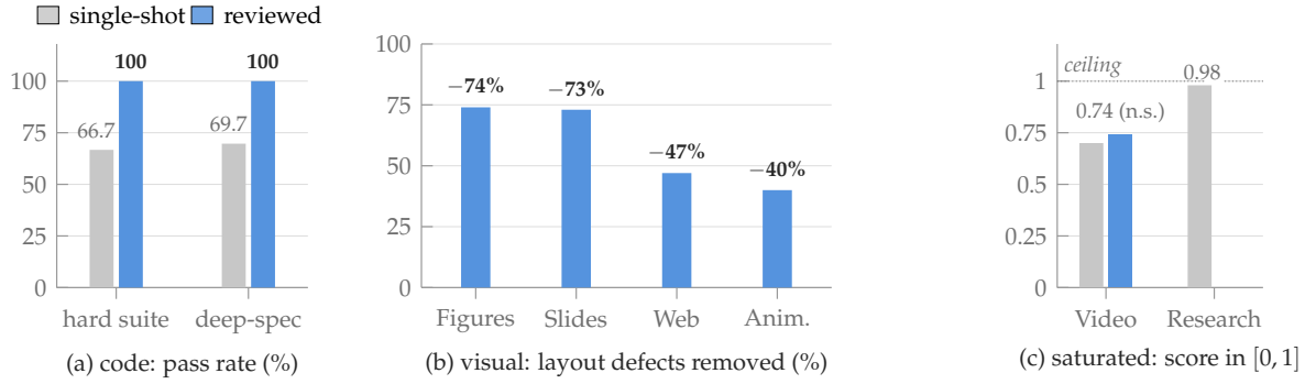
Figure 2. Results at a glance: one grounded loop, seven modalities. (a) Execution feedback lifts both code suites to a strict 100% pass rate, recovering every single-shot failure (3-seed means; Section 4). (b) Grounded geometry feedback removes 40–74% of the layout defects a deterministic DOM instrument measures, on all four visual modalities (every reduction statistically decisive; Section 6). (c) The two remaining modalities are scoped negatives: video editing is already strong single-shot (the reviewed lift is not significant), and deep research saturates at 0.98 single-shot factual accuracy, leaving no headroom for feedback to claim (Section 6).
