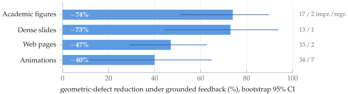
Figure 11. Grounded geometric feedback removes real layout defects on all four visual modalities. Mean defect reduction under one identical configuration (3 seeds; whiskers are paired-bootstrap 95% CIs, all excluding zero; right column counts improved vs. regressed task-runs; all paired sign tests p < 2 \times 10^{-3} ; full statistics in Table 6). The standard VLM-on-a-screenshot metric measures none of this.
