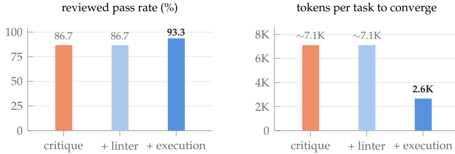
Figure 8. Swapping only the feedback signal on a fixed code suite: improvement tracks coverage, and cost tracks it decisively. One reviewing pass per configuration. Ungrounded critique (orange), critique + linter (light blue: grounded, but observing only form ), and critique + test execution (blue: grounded, observing behavior ). The linter configuration matches bare critique on these runtime-logic bugs (exactly what the coverage principle predicts) while the execution configuration reaches a higher ceiling at \sim 2.5\times lower cost and fewer iterations (1.53 vs. 2.07; per-seed detail in Table 4).
