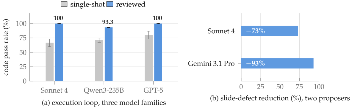
Figure 12. Both grounded loops replicate across model families. (a) Single-shot vs. harness-reviewed code pass rate for three families, three seeds each (lifts +33.3/+22.2/+20.0 pp; whiskers \pm 1 SD across seeds). The reviewed bars carry zero seed variance for all three families. (b) The deterministic geometric loop on dense real-paper slides, scored by the same model-free DOM instrument, reproduces with Gemini 3.1 Pro as proposer and is larger there (19 of 20 decisive task-runs improve): Gemini starts more defect-prone and the loop removes almost all of the excess.
