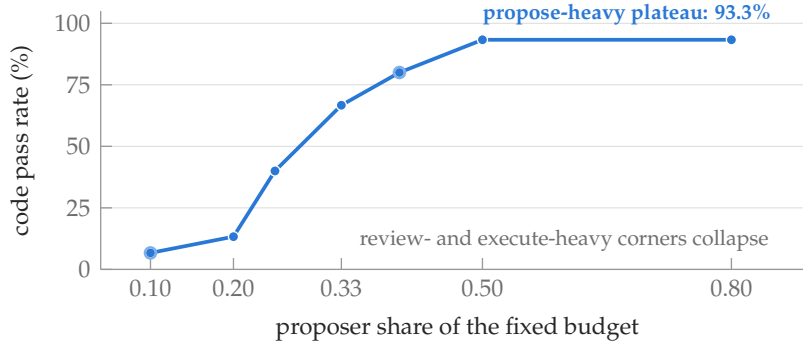
Figure 13. Pass rate is monotone in the proposer’s budget share. Nine allocations of a fixed 10K-token budget across proposer / execution / reviewer, on the hard code suite (open markers: a second allocation with the same proposer share but a different execution/review split, showing that the proposer share alone predicts the outcome). The spread across the sweep is 86.6 pp; full simplex in Table 9.
