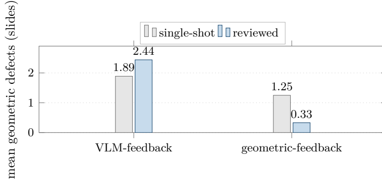
Figure 6: An ungrounded reviewer makes layout worse (controlled ablation). Same modality, same proposer; only the reviewer’s grounding varies. A VLM-feedback reviewer increases mean geometric defects ( 1.89 \rightarrow 2.44 ); the deterministic geometric-feedback reviewer reduces them ( 1.25 \rightarrow 0.33 ). The grounded signal is necessary on the feedback side, not just the metric side.
