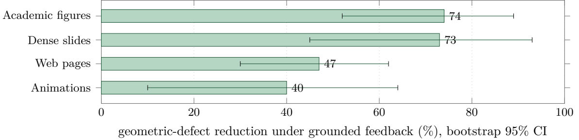
Figure 6: Grounded geometric feedback removes real layout defects on all four visual modalities (mean reduction, with whiskers the paired-bootstrap 95% CIs, all excluding zero). The standard VLM-on-a-screenshot metric measures none of this.
