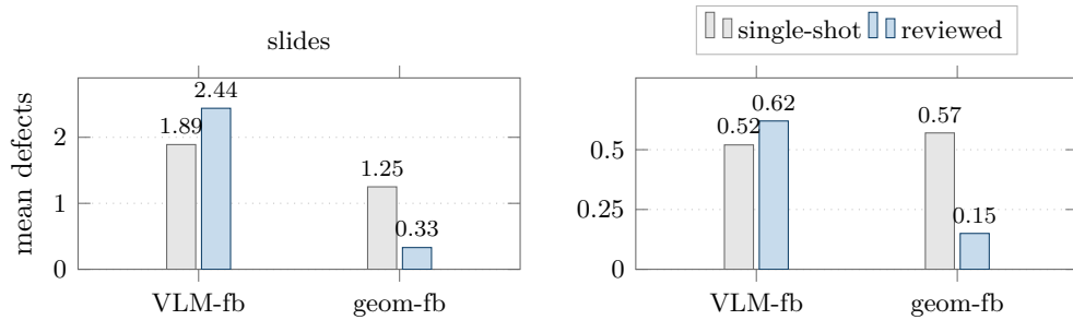
Figure 7: An ungrounded reviewer fails to fix layout, while a grounded one does (controlled ablation, two modalities) . Same task suite and proposer model, with only the reviewer’s grounding varying. The two arms are separate runs, so each is plotted against its own single-shot (hence the differing single-shot bars). The VLM-feedback reviewer (VLM-fb) does not reduce defects and on slides increases them (slides 1.89 \rightarrow 2.44, figures 0.52 \rightarrow 0.62, directional/n.s.). The deterministic geometric-feedback reviewer (geom-fb) reduces them (slides 1.25 \rightarrow 0.33, figures 0.57 \rightarrow 0.15). The grounded signal is necessary on the feedback side, not just the metric side.
