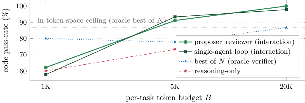
Figure 2: Two in-token-space axes saturate. Interaction does not. Measured code pass-rate vs. per-task token budget on the 15 hard tasks (3-seed means, full table with SDs in Table 3). Reasoning-only plateaus at its information ceiling (73.3%), and best-of- N plateaus at 86.7% even with an oracle (ground-truth) verifier (dotted). Both are functions of the frozen (\Theta, X) and flatten with budget, the latter at the high-probability support of the proposer’s own output distribution. The two feedback-iterating strategies instead climb past the oracle-sampling ceiling to \geq 97.8\% (harness: strict 100%), importing information from execution each cycle, the DPI prediction made concrete. These are measured points, not a schematic.
