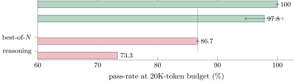
Figure 3: Two axes saturate. The third does not. The 20K-token snapshot of Figure 2: the two in-token-space axes (red) plateau below the interaction strategies (green), which all reach \geq 97.8\% . Whiskers are \pm 1 SD over three seeds (reasoning was run once): the single-agent loop carries seed variance ( \pm 3.1 pp, 100% in 2 of 3 seeds) while the proposer-reviewer harness reaches strict 100% with zero seed variance. Dotted line: oracle best-of- N ceiling.
