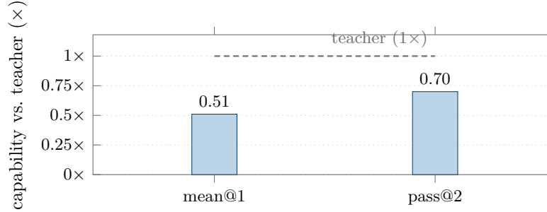
Figure 9: An 8B student internalizes most of the teacher’s interaction quality. Distilled 8B markdown student as a fraction of the frontier teacher on the 44-task OOD suite (Table 12): a single sample recovers 0.51\times and two samples 0.70\times of teacher capability (sampling closes the gap), at \sim 10\times lower deployment cost. On the 18-task hard held-out suite the same student passes 44%/56% at pass@1/pass@3.
