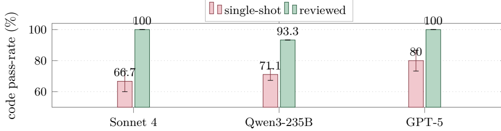
Figure 8: The execution-grounded loop helps every model family. Single-shot vs. harness-reviewed code pass-rate for three model families, each over three independent on-policy seeds (+33.3/+22.2/+20.0 pp). Whiskers are \pm 1 SD across seeds. The reviewed bars carry zero seed variance for all three families.
