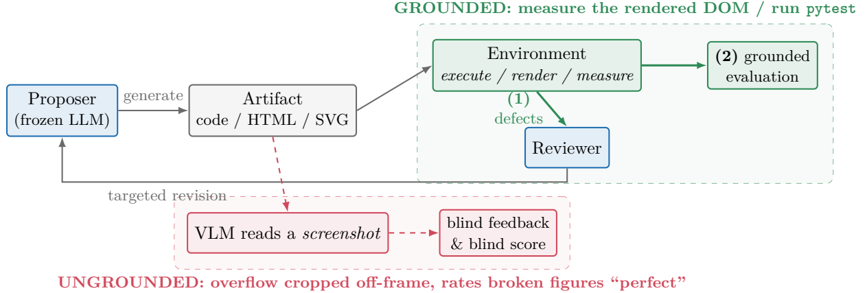
Figure 1: Grounding must hold on both sides of the interaction loop. A proposer emits an artifact, and a grounded environment executes/renders/measures it. That same observation does double duty. (1) As grounded feedback , it becomes a defect list the reviewer turns into a targeted revision, the channel that lets interaction import information from outside the weights and exceed the reasoning/sampling ceiling (Section 3). (2) As grounded evaluation , it is the score that makes the gain measurable. Substituting the default VLM-on-a-screenshot judge (red lane) breaks both : it is structurally blind to off-canvas overflow and fine overlap, so it neither scores the defect nor (as a reviewer) fixes it.
