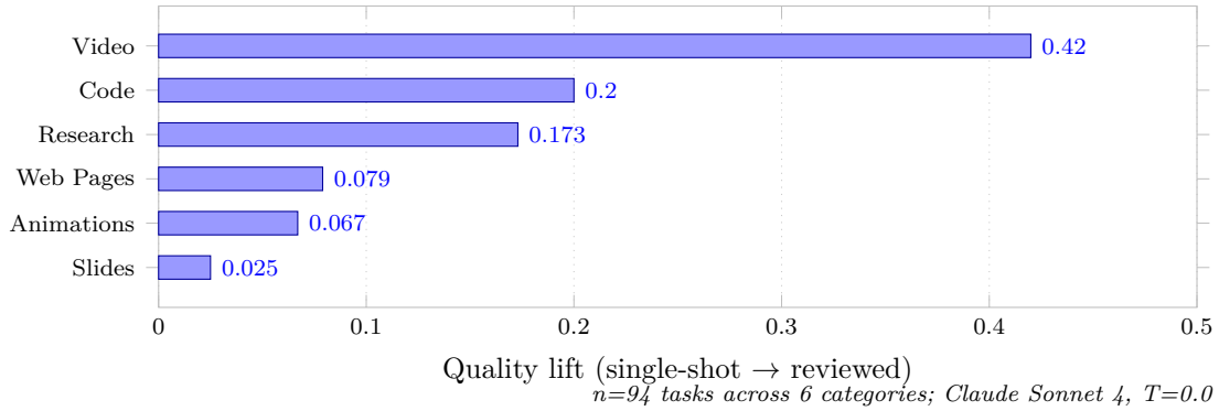
Figure 5: Phase 1 baseline (single-run): interaction-scaling lift orders by feedback actionability . Execution feedback (Code: +0.20, Video: +0.42) is binary and machine-readable; factual verification (Research: +0.17) is specific but softer; visual feedback (Web: +0.08, Animations: +0.07, Slides: +0.03) is holistic and lossy to operationalize. The multi-run averages reported in Table 2 reorder some within-tier rows but preserve the top-tier gap.
