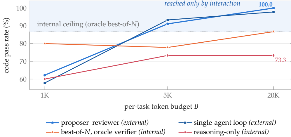
Figure 5. Internal scaling saturates; external scaling does not (P1). Code pass rate vs. per-task token budget on the 15 hard tasks (3-seed means; full table in Table 2). Both internal strategies flatten as the budget grows: reasoning-only at its information ceiling, and best-of- N at 86.7% even with an oracle (ground-truth-test) verifier, capped by the high-probability part of the model’s own output distribution. The two external strategies import execution feedback each cycle and climb past that ceiling, the proposer-reviewer harness to a strict 100% with zero seed variance. We run this experiment in Section 4.
