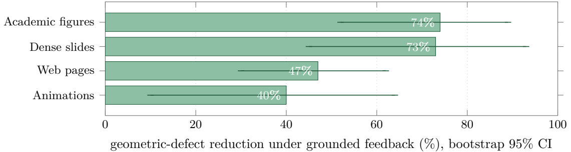
Figure 6. Grounded geometric feedback removes real layout defects on all four visual modalities (mean reduction, with whiskers the paired-bootstrap 95% CIs, all excluding zero). The standard VLM-on-a-screenshot metric measures none of this.
