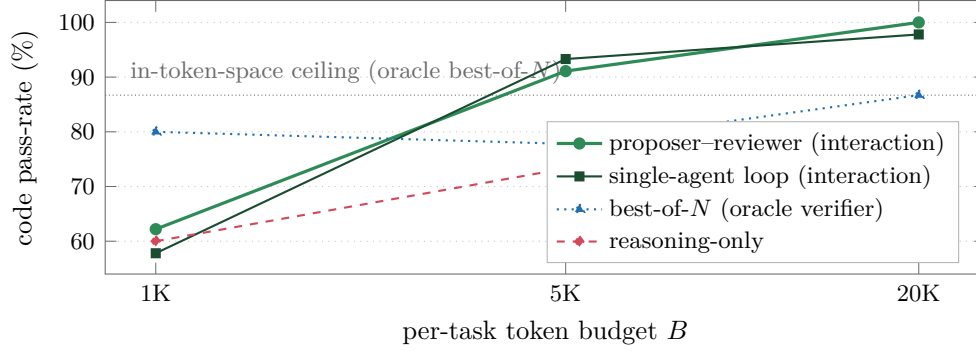
Figure 2. Two in-token-space axes saturate. Interaction does not. Measured code pass-rate vs. per-task token budget on the 15 hard tasks (3-seed means, full table with SDs in Table 3). Reasoning-only plateaus at its information ceiling (73.3%), and best-of- N plateaus at 86.7% even with an oracle (ground-truth) verifier (dotted). Both are functions of the frozen (\Theta, X) and flatten with budget, the latter at the high-probability support of the proposer’s own output distribution. The two feedback-iterating strategies instead climb past the oracle-sampling ceiling to \geq 97.8\% (harness: strict 100%), importing information from execution each cycle, the DPI prediction made concrete. These are measured points, not a schematic.
