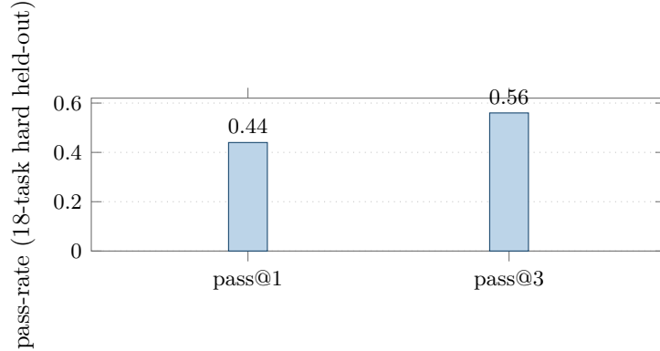
Figure 8: An 8B student internalizes interaction quality. Pass@1/pass@3 of the distilled 8B markdown student on the hard held-out suite ( 0.50\times/0.70\times teacher mean@1/@2 on the 44-task OOD set), at \sim 10\times lower deployment cost.
