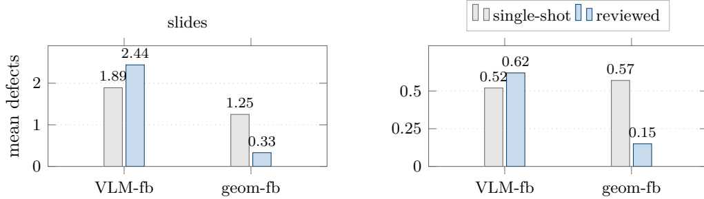
Figure 6: An ungrounded reviewer makes layout worse (controlled ablation, two modalities). Same tasks and proposer; only the reviewer’s grounding varies. A VLM-feedback reviewer (VLM-fb) increases mean geometric defects on both slides (1.89 \rightarrow 2.44) and figures (0.52 \rightarrow 0.62); the deterministic geometric-feedback reviewer (geom-fb) reduces them (1.25 \rightarrow 0.33; 0.57 \rightarrow 0.15). The grounded signal is necessary on the feedback side, not just the metric side.
