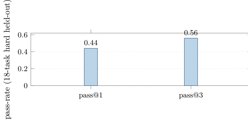
Figure 8: An 8B student internalizes interaction quality. Pass@1/pass@3 of the distilled 8B markdown student on the hard held-out suite ( 0.50\times/0.70\times teacher mean@1/@2 on the 44-task OOD set), at \sim 10\times lower deployment cost.
