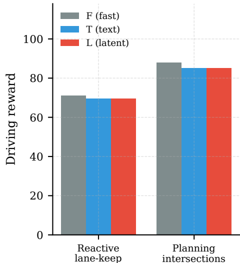
MetaDrive: slow adds nothing, even with planning
