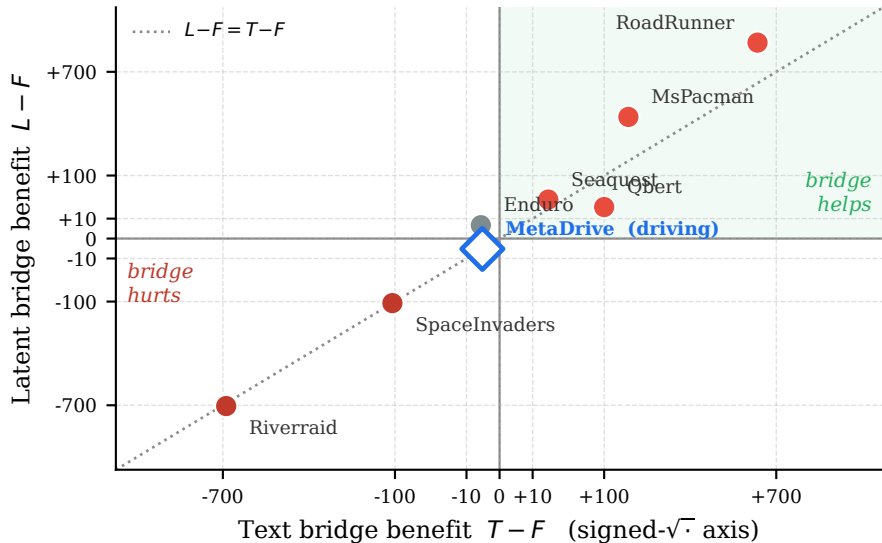
Latent helps iff slow reasoning helps ( r = 0.97, n = 8 )
