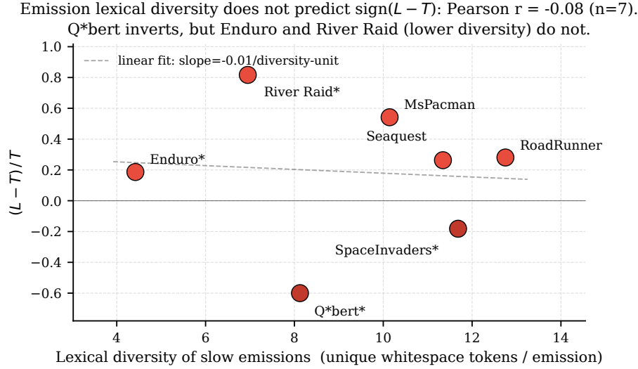
Figure 11. Emission statistics do not predict the sign of L - T ( n = 7 ). x = mean unique whitespace tokens per slow emission (seed-0 T -trajectory). y = (L - T) / T . Q*bert is the only y < 0 point with a large T , but Enduro and River Raid (lower diversity) have y > 0 , and SpaceInvaders (high diversity) is mildly y < 0 . Pearson r = -0.08 . The dashed line is the linear fit and is shown only to make the lack of structure visible.
