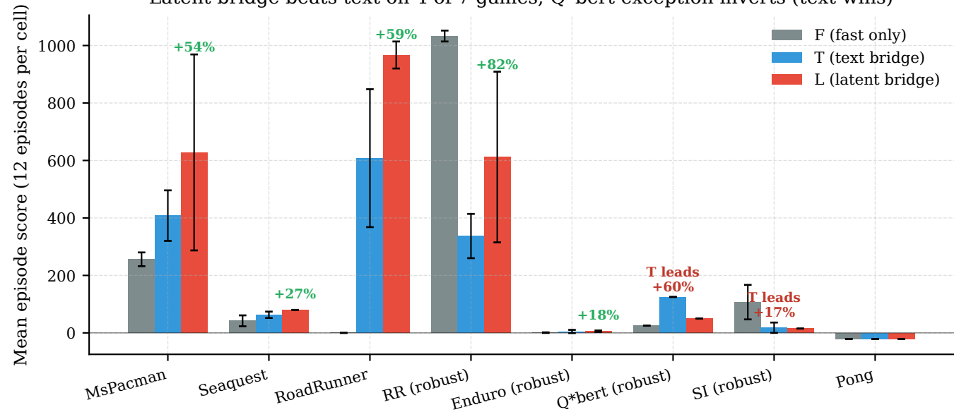
Latent bridge beats text on 4 of 7 games; Q*bert exception inverts (text wins)
