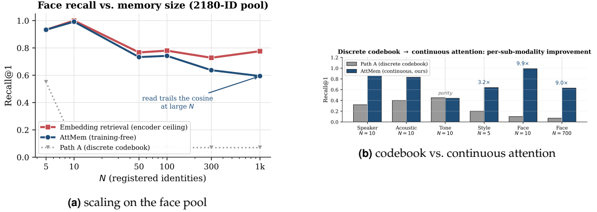
Figure 17. Left: on the face pool the training-free read ties the encoder ceiling at small N and trails it at N \geq 300 (the encoder-ceiling inversion, Table 9), both declining gracefully, while the codebook predecessor never gets off the floor. Right: continuous attention beats the discrete codebook 2–10 \times on every sub-modality.
