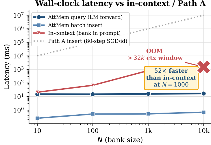
Figure 5. Recall latency is flat in bank size ( \sim 15 ms, dominated by the frozen model’s own forward pass) and insertion is \mathcal{O}(1) . Feeding the same registered perceptions in as context grows linearly and exhausts the 32k context window (Qwen2.5-3B) at ten thousand identities. Per-concept fine-tuning (PATH A-style) costs gradient steps per identity. Log-log axes.
