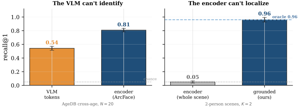
Figure 2. Neither component works alone; grounding cover both blind spots. Two targeted experiments isolating the failures of each component. Left (identity) : on AgeDB cross-age faces ( N=20 ), the VLM’s vision tokens are a weak identity encoder (recall 0.54) while a dedicated face encoder achieves 0.81 recall. Right (localization) : in two-person scenes ( K=2 ), the performance of a bare encoder embedding the whole scene is close to random (0.05), while grounding the referent first achieves near-perfect performance (0.96). The division of labour is essential: the VLM excels at localization but struggles with identity invariance, while the specialist encoder is highly invariant but cannot locate the target. Detailed ablations appear in Figure 7.
