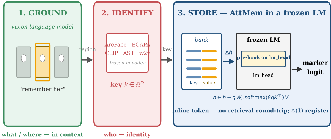
Figure 1. A vision-language model grounds the referent the user means in a cluttered scene ( what/where ); a purpose-built encoder turns the grounded region into an identity key ( who ); and ATTMem stores the key on a frozen language model, reading it back as a single inline token. Neither component suffices alone — the VLM is a weak identity encoder, and a bare encoder cannot pick the referent out of a scene; grounded, they recover the correct-region oracle (Figure 2). The mechanism is detailed in Figure 4.
