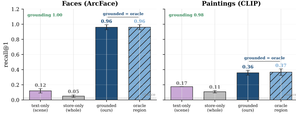
Figure 7. Ablation of the grounded memory on cluttered scenes ( M=40 , two referents per scene). Performance increases left to right: text-only , where the VLM describes the referent from the whole scene and the captions are matched; store-only , where the whole scene is embedded with no grounding; grounded , our ground + identify + store strategy; and the correct-region oracle . Both text-only and store-only perform near random guessing, while grounding reaches the oracle-level performance. Retrieval uses the encoder’s nearest neighbor in all cases, so the large gain comes from grounding itself, not the matching method. Faces: ArcFace with landmark alignment, 5 seeds; paintings: CLIP with no alignment, 3 seeds. Error bars show \pm 95\% CI.
