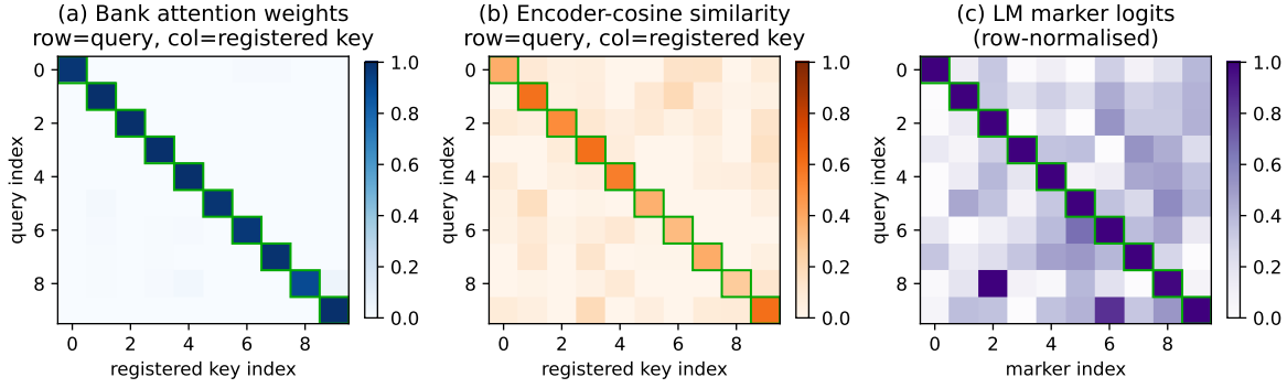
Figure 12. One recall, three views (held-out faces, ten identities). (a) With a sharp temperature, attention over the memory bank forms a near-pure diagonal (average 0.98), strongly committing to the top encoder match. (b) The underlying encoder cosine similarities show a softer diagonal (avg. 0.46) with noticeable off-diagonal mass; the memory faithfully inherits these similarities and their errors. (c) The resulting marker logits keep the correct identity at the top. Overall, the attention faithfully reads the encoder’s nearest neighbour as a token; it does not sharpen the similarity.
