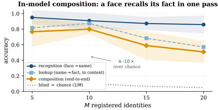
Figure 13. In-model composition: we register M faces with dedicated name markers, bind one fact per name in context, then then query the associated fact using a held-out cross-condition photo, all in one forward pass. End-to-end accuracy (gold) closely tracks the product of recognition accuracy (navy) times the model’s in-context lookup accuracy (blue) and beats the face-withheld random chance baseline by 4–10 \times . Results averaged over 12 draws; bands show \pm one standard deviation.
