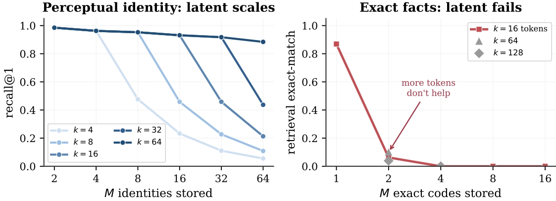
Figure 15. Two capacity laws for memory compressed into k soft tokens read by a frozen language model, the mechanism behind the router. Left: Perceptual identity is capacity-limited. When compressing M faces into k prototype slots and querying with a cross-condition sample, recall scales as \approx \min(1, k/M) \times C(M) where C(M) is the encoder ceiling ( \approx 1 for faces). Voices follow the same pattern. One slot per identity recovers full encoder performance, and more slots allow more identities to be stored. Right: Exact factual content is binding-limited. A latent can reliably hold and retrieve a single exact code (0.87), but attempting to store and retrieve multiple codes collapses immediately (0.06 at two codes), and adding more latent tokens does not help. Recognition scales with the latent budget while exact recall does not, which is why it belongs in a text store.
