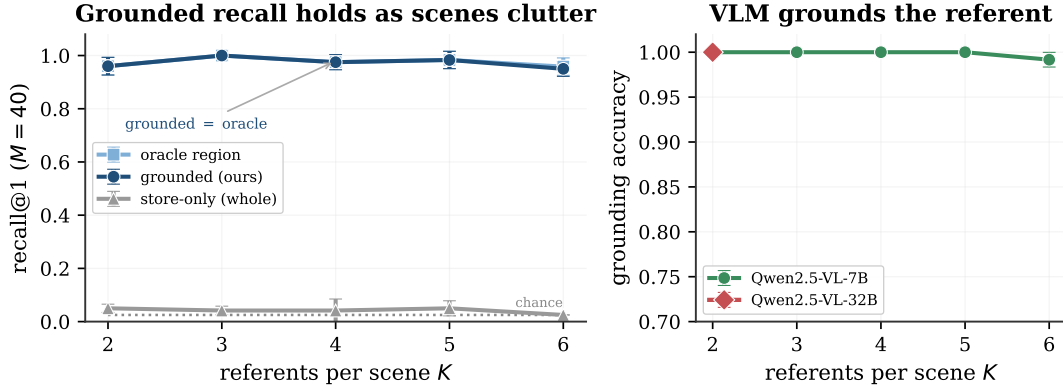
Figure 8. The grounded advantage is robust to scene clutter and VLM scale (faces, M=40 ). Left: As referents per scene grow from two to six, grounded recall (navy) closely tracks the correct-region oracle (light blue, nearly coincident), while whole-scene recall remains near the floor. Right: Grounding accuracy stays at 1.00 through K=5 and only drops slightly to 0.99 at K=6 . Performance is identical for Qwen2.5-VL-7B and Qwen2.5-VL-32B, showing that the decomposition does not require a large grounding model.
