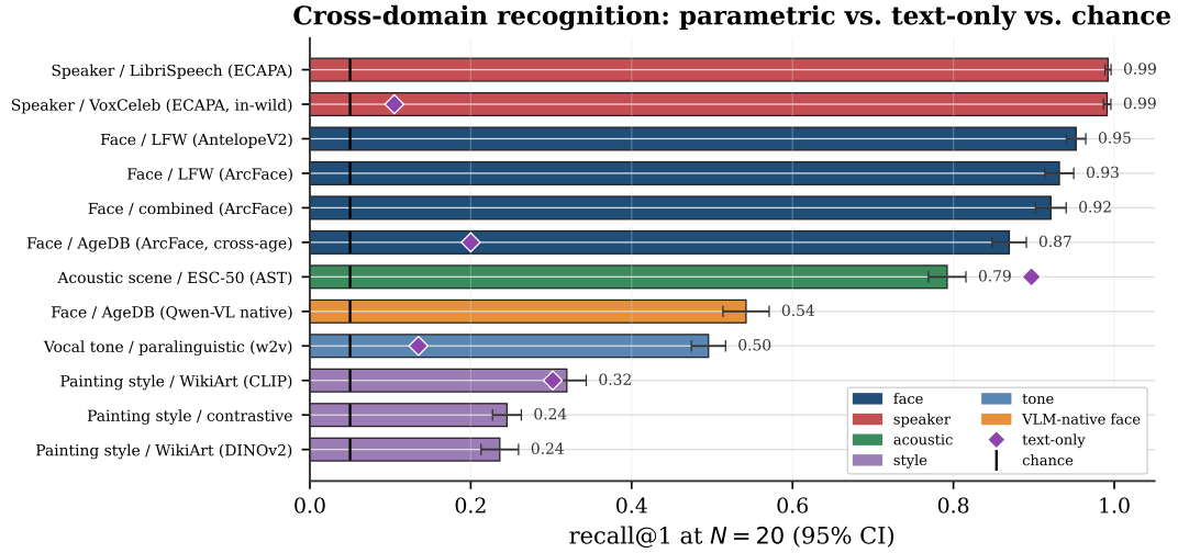
Figure 7. The recognition core across 12 perceptual domains and 5 modalities (1,080 tasks; recall@1 at N=20 , 30 draws, 95% CI), coloured by modality, against chance ( 1/N , black ticks) and the text-only caption baseline where measured (purple diamonds, per modality). Parametric recall tracks the encoder and clears chance everywhere, far exceeding text-only on perceptual identity (speaker, face, tone). The one inversion is the nameable acoustic scene, where a caption (“typing on a keyboard”) edges the weaker AST encoder — exactly the router boundary (§7): text suffices for nameable categories, the parametric bank for identity. The VLM’s own native vision encoder (orange) reads the same AgeDB faces far below a purpose-built one.
