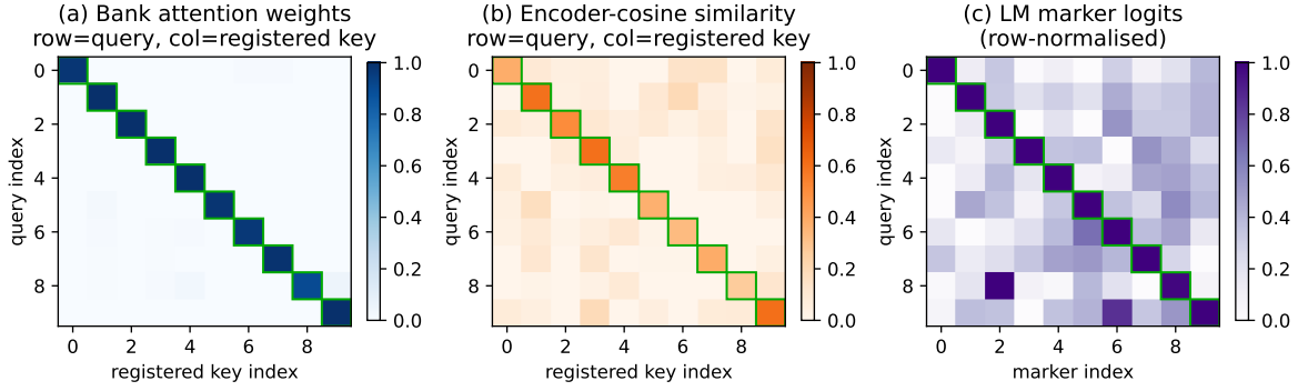
Figure 8. One recall, three views (held-out faces, ten identities). (a) with a sharp temperature, bank attention is a near-pure diagonal (avg. 0.98), committing to the top encoder match. (b) the underlying encoder cosine has a softer diagonal (avg. 0.46) with off-diagonal mass; the memory inherits whatever errors live here. (c) the resulting marker logits keep the argmax identity on top. The attention faithfully reads the encoder’s nearest neighbour as a token; it does not sharpen the similarity.
