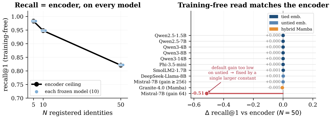
Figure 11. The training-free read reproduces the encoder on every frozen model, the supporting property behind the “store” step. Left: each model’s training-free recall lands on the encoder ceiling (paired, 20 draws). Right: the gap from the encoder at N=50 is \approx 0 across ten families (1.5B–14B, tied and untied embeddings, hybrid-Mamba); only an untied model at the default gain dips (red), fixed by a single larger read-strength constant. No gradient steps anywhere.
