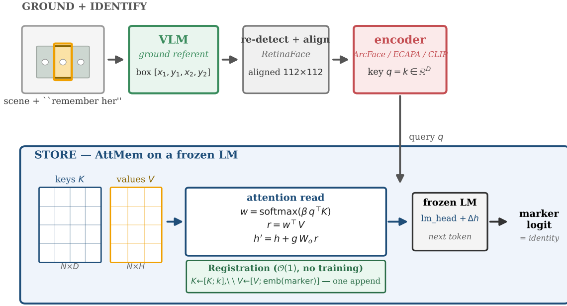
Figure 3. The grounded memory in detail. Ground + identify (top): the VLM resolves the referent to a box, a modality detector re-detects and aligns the region (RetinaFace for faces), and a frozen perceptual encoder (ArcFace / ECAPA / CLIP) maps it to an L2-normalized key q=k \in \mathbb{R}^D . Store (bottom): ATTMEM holds keys K ( N \times D ) and values V ( N \times H , the model’s own marker-token embeddings); the attention read w=\text{softmax}(\beta q^\top K) , r=w^\top V , h'=h+g W_o r adds a residual at the output head that biases the next token toward the matching marker. The read has no trainable parameters ( \beta, g are constants); registration is a single \mathcal{O}(1) append.
