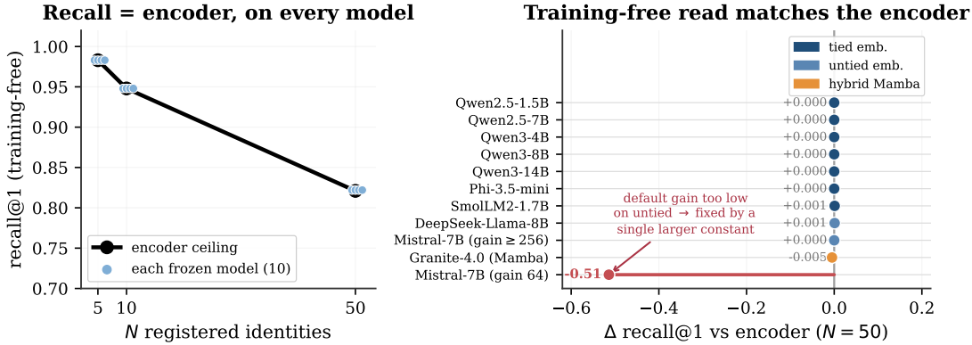
Figure 15. The training-free read reproduces the encoder on every frozen model, the supporting property behind the “store” step. Left: each model’s training-free recall lands on the encoder ceiling (paired, 20 draws). Right: the gap from the encoder at N=50 is \approx 0 across ten families (1.5B–14B, tied and untied embeddings, hybrid-Mamba); only an untied model at the default gain dips (red), fixed by a single larger read-strength constant. No gradient steps anywhere.
