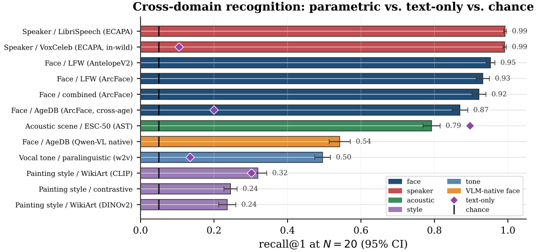
Figure 9. The recognition core across 12 perceptual domains and 5 modalities (1,080 tasks; recall@1 at N=20 , 30 draws, 95% CI), coloured by modality, against chance ( 1/N , black ticks) and the text-only caption baseline where measured (purple diamonds, per modality). Parametric recall tracks the encoder and clears chance everywhere, far exceeding text-only on perceptual identity (speaker, face, tone). The one inversion is the nameable acoustic scene, where a caption (“typing on a keyboard”) edges the weaker AST encoder — exactly the router boundary (§7): text suffices for nameable categories, the parametric bank for identity. The VLM’s own native vision encoder (orange) reads the same AgeDB faces far below a purpose-built one.
