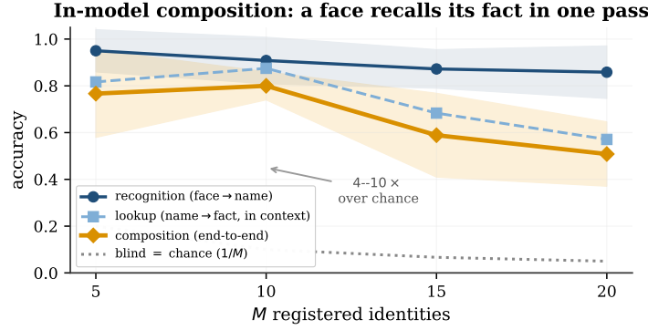
Figure 12. In-model composition: register M faces with name markers, bind one fact per name in context, then recall the fact from a held-out cross-condition photo, all in one forward pass. End-to-end accuracy (gold) tracks recognition (navy) times the model’s in-context lookup (blue) and beats the face-withheld chance baseline by 4–10 \times . 12 draws; bands are \pm std.
