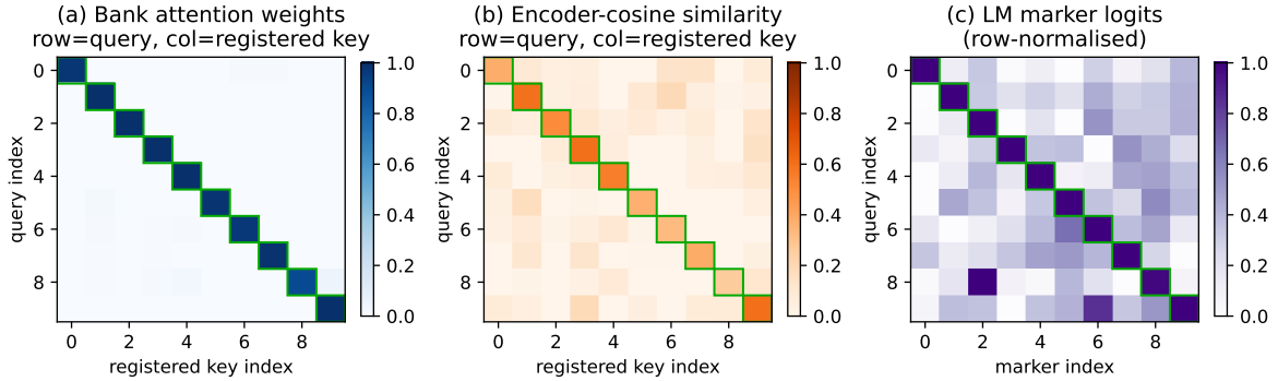
Figure 11. One recall, three views (held-out faces, ten identities). (a) with a sharp temperature, bank attention is a near-pure diagonal (avg. 0.98), committing to the top encoder match. (b) the underlying encoder cosine has a softer diagonal (avg. 0.46) with off-diagonal mass; the memory inherits whatever errors live here. (c) the resulting marker logits keep the argmax identity on top. The attention faithfully reads the encoder’s nearest neighbour as a token; it does not sharpen the similarity.
