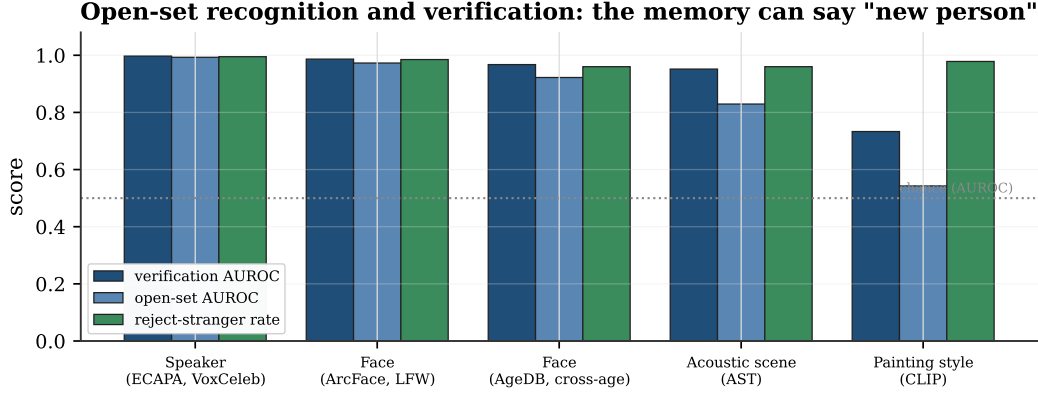
Figure 10. Beyond closed-set recall, the memory verifies identities and rejects strangers ( N=20 enrolled, 30 draws). Per modality: verification AUROC (same vs different identity), open-set AUROC (enrolled vs never-enrolled probe), and the reject-stranger rate at the balanced threshold. All are high where the encoder is strong (voice, face) and fall where it is weak (painting style), the same dependence as recall.
