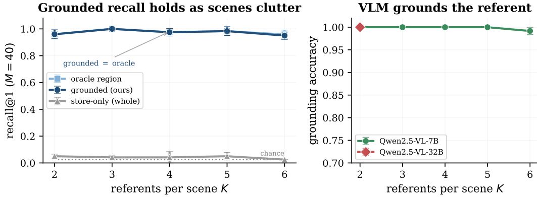
Figure 7. The grounded advantage is robust to scene clutter and grounder scale (faces, M=40 ). Left: as referents per scene grow from two to six, grounded recall (navy) stays at the correct-region oracle (light blue, coincident) while whole-scene recall stays at the floor. Right: grounding accuracy stays at 1.00 through K=5 and dips only to 0.99 at K=6 , and is identical for Qwen2.5-VL-7B and -32B, so the decomposition does not require a large grounder.
