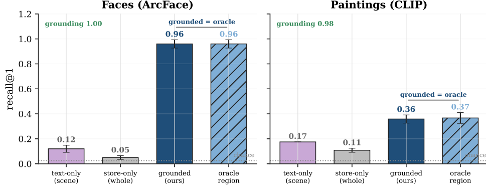
Figure 6. Ablation of the grounded memory on cluttered scenes ( M=40 , two referents per scene). Capability increases left to right: text-only , where the VLM describes the referent from the whole scene and captions are matched; store-only , embedding the whole scene with no grounding; grounded (ground + identify + store, ours); and the correct-region oracle . Both text-only and store-only are near chance, while grounding recovers the oracle. Retrieval coincides with store throughout (both are the encoder’s nearest neighbour), so the gain is grounding, not the matcher. Faces: ArcFace, landmark alignment, 5 seeds; paintings: CLIP, no alignment, 3 seeds; error bars \pm 95\% CI.
