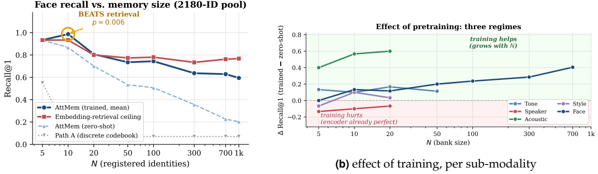
Figure 9. Left: parametric memory beats retrieval at small memories and degrades gracefully; the codebook predecessor never gets off the floor. Right: training helps most where the encoder is imperfect, and slightly hurts where it is already perfect.
