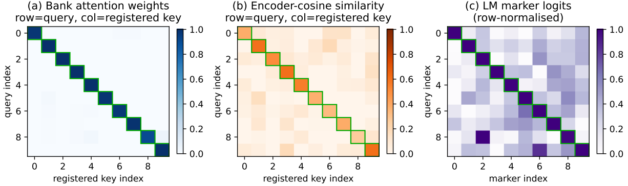
Figure 4: What the mechanism does , on a held-out face cross-condition probe ( N=10 ). (a) Bank attention weights: a sharp diagonal — each query attends overwhelmingly to its correct target identity. (b) Encoder cosine similarity: diagonal-dominant but with off-diagonal noise (the source of RAG’s errors). (c) LM marker logits (row-normalised): inherit the attention diagonal plus LM value-side adjustments that further sharpen the argmax. The value-side space is where the surplus discriminative signal over encoder cosine comes from.
