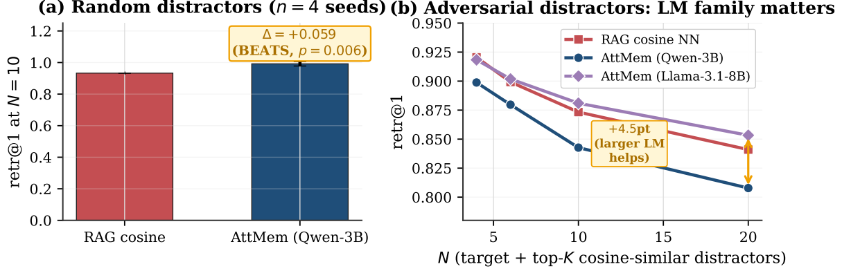
Figure 12: Random vs adversarial distractors. (a) On random banks at N=10 , AttMem beats RAG by 5.9 pp ( p=0.006 , n=4 ). (b) On adversarial banks: with Qwen-3B, standard-trained AttMem trails RAG by 2–3 pp; with Llama-3.1-8B, AttMem matches or beats RAG at K \geq 5 . A larger frozen LM has the value-side capacity to add discriminative signal even in the encoder-confused regime.
