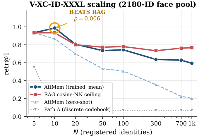
Figure 5: V-XC-ID-XXXL scaling. Parametric memory (trained, 12K-step curriculum) beats embedding-RAG at N=10 ( p=0.006 , n=4 ; shaded \pm SEM) and tracks within \sim 17 pp through N=1000 . Zero-shot AttMem falls off rapidly at N \geq 50 . Path A saturates at \sim 0.07 regardless of N , encoder, or compute.
