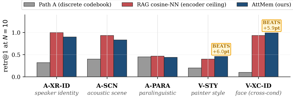
Figure 3: PerceptMem v0.2 scorecard at N=10 . The parametric multimodal memory (navy) exceeds the embedding-RAG cosine-NN baseline on V-XC-ID ( p=0.006 , n=4 ) and V-STY ( p=0.009 , n=5 ), ties it on A-PARA (0.47 vs 0.47), and trails it by \sim 10 pp on A-SCN (0.83 vs 0.93) and A-XR-ID (0.90 vs 1.00, where the encoder is already perfect). The discrete-codebook predecessor (Path A, grey) is 2\text{--}10\times lower across all sub-modalities. Labels show the percentage-point gap over RAG.
