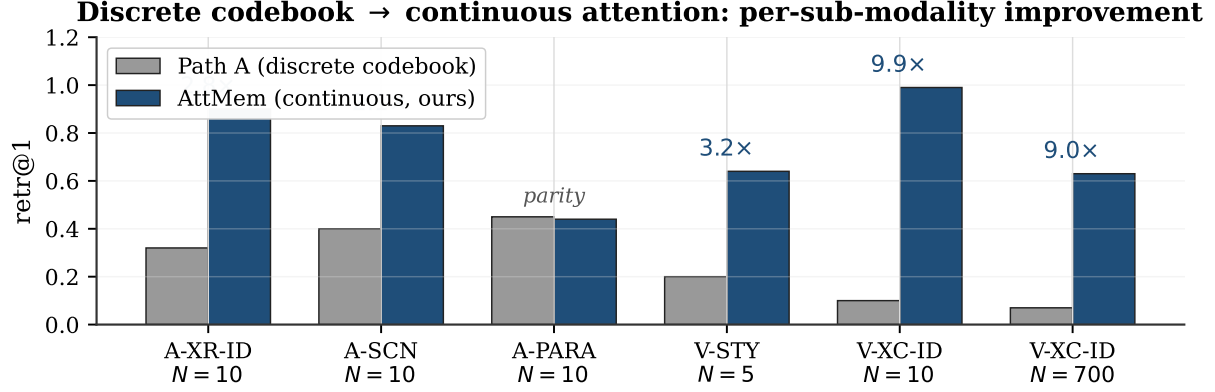
Figure 6: Discrete codebook → continuous attention. Replacing the codebook with continuous attention over the (key, value) bank yields 2–10× retr@1 per sub-modality. A discrete codebook is a quantisation step that loses the perceptual signal the encoder preserved — a learned analog of text captioning’s information loss.
