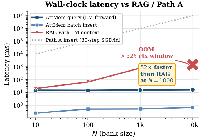
Figure 7: Wall-clock latency (Qwen2.5-3B, H100-class GPU). Parametric-memory query is flat ~15 ms (bank matmul is microseconds; LM forward dominates). Batch insertion is ~0.5 ms total. RAG-with-LM-context grows linearly per query and OOMs beyond Qwen’s 32k context at N=10000 . Path A insertion is ~1 s/id (80-step SGD; off the top at scale).
