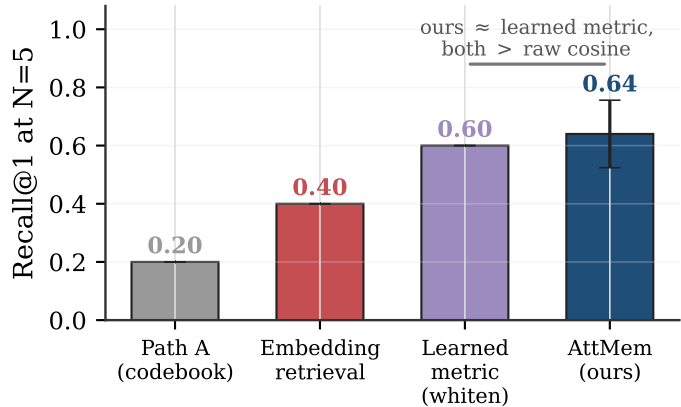
Painter-style recall (CLIP encoder)
