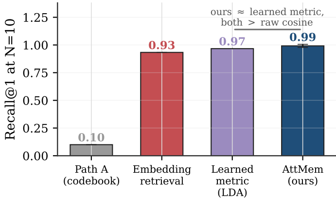
Face recall (2180-identity pool)
