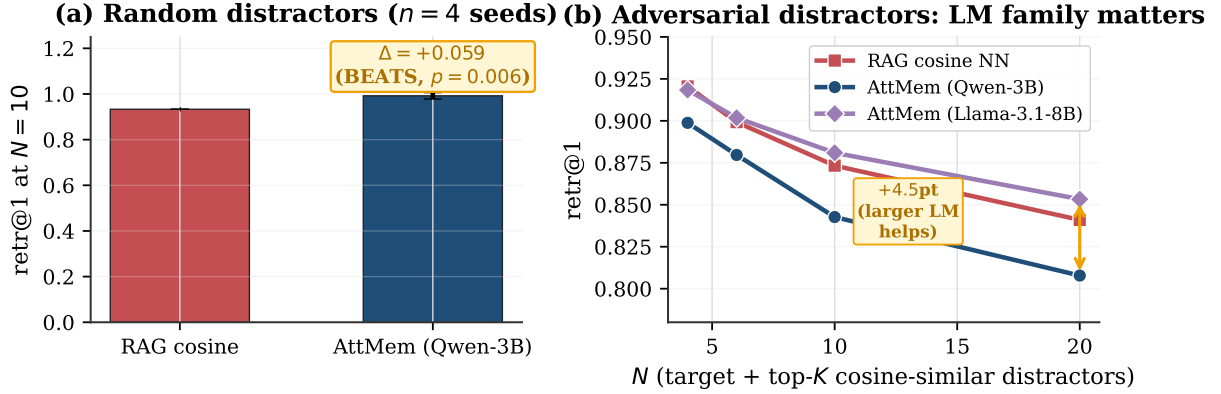
Figure 9: Random vs adversarial distractors. (a) On random bank composition at N=10 , AttMem BEATS RAG by 5.9 pp ( p=0.006 , n=4 seeds). (b) On adversarial banks (target + top-K cosine-similar distractors): with Qwen-3B, RAG cosine wins by 2–3 pp; with Llama-3.1-8B, AttMem matches or BEATS RAG at K \geq 5 . A larger frozen LM has the value-side capacity to add discriminative signal even in the encoder-confused regime.
