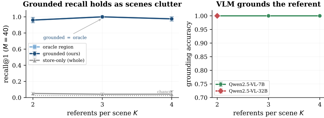
Figure 6. The grounded advantage is robust to scene clutter and grounder scale (faces, M=40 ). Left: as referents per scene grow from two to four, grounded recall (navy) stays at the correct-region oracle (light blue, coincident) while whole-scene recall stays at the floor. Right: grounding accuracy is 1.00 at every clutter level and identical for Qwen2.5-VL-7B and -32B, so the decomposition does not require a large grounder.
