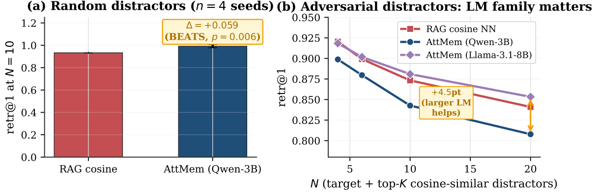
Figure 11: Random vs adversarial distractors. (a) On random bank composition at N=10 , AttMem BEATS RAG by 5.9 pp ( p=0.006 , n=4 seeds). (b) On adversarial banks: with Qwen-3B, standard-trained AttMem trails RAG by 2–3 pp; with Llama-3.1-8B, AttMem matches or BEATS RAG at K \geq 5 . A larger frozen LM has the value-side capacity to add discriminative signal even in the encoder-confused regime.
