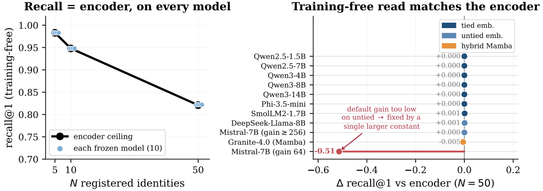
Figure 13. The training-free read reproduces the encoder on every frozen model, the supporting property behind the “store” step. Left: each model’s training-free recall lands on the encoder ceiling (paired, 20 draws). Right: the gap from the encoder at N=50 is \approx 0 across ten families (1.5B–14B, tied and untied embeddings, hybrid-Mamba); only an untied model at the default gain dips (red), fixed by a single larger read-strength constant. No gradient steps anywhere.
