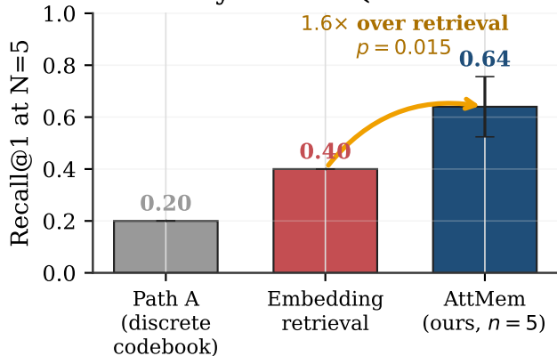
Painter-style recall (CLIP encoder)
