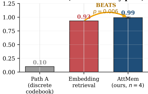
Face recall (2180-identity pool)
