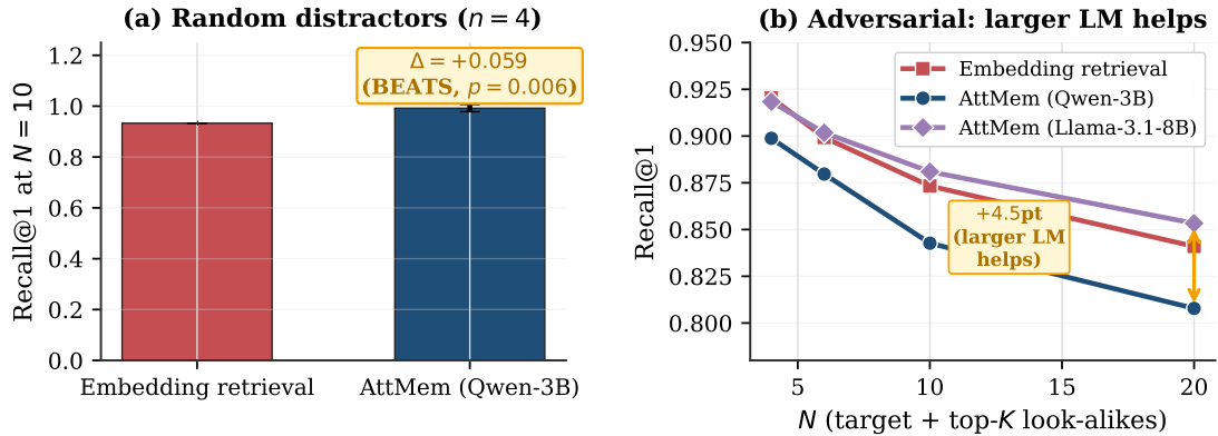
Figure 9. Random vs. adversarial distractors. (a) on random banks, parametric memory beats retrieval by 5.9 points ( p=0.006 ). (b) on adversarial banks, a small frozen model (Qwen-3B) trails retrieval by a few points under standard training, while a larger one (Llama-3.1-8B) matches or beats it even without look-alike training. The larger model has more representational room to discriminate when the encoder is confused.
