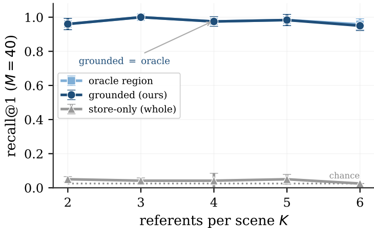
Grounded recall holds as scenes clutter
