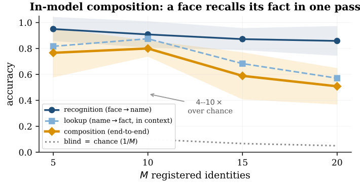
Figure 13. In-model composition: we register M faces with dedicated name markers, bind one fact per name in context, then query the associated fact using a held-out cross-condition photo, all in one forward pass. End-to-end accuracy (gold) closely tracks the product of recognition accuracy (navy) times the model’s in-context lookup accuracy (blue) and beats the face-withheld random chance baseline by 4–10 \times . Results averaged over 12 draws; bands show \pm one standard deviation.
