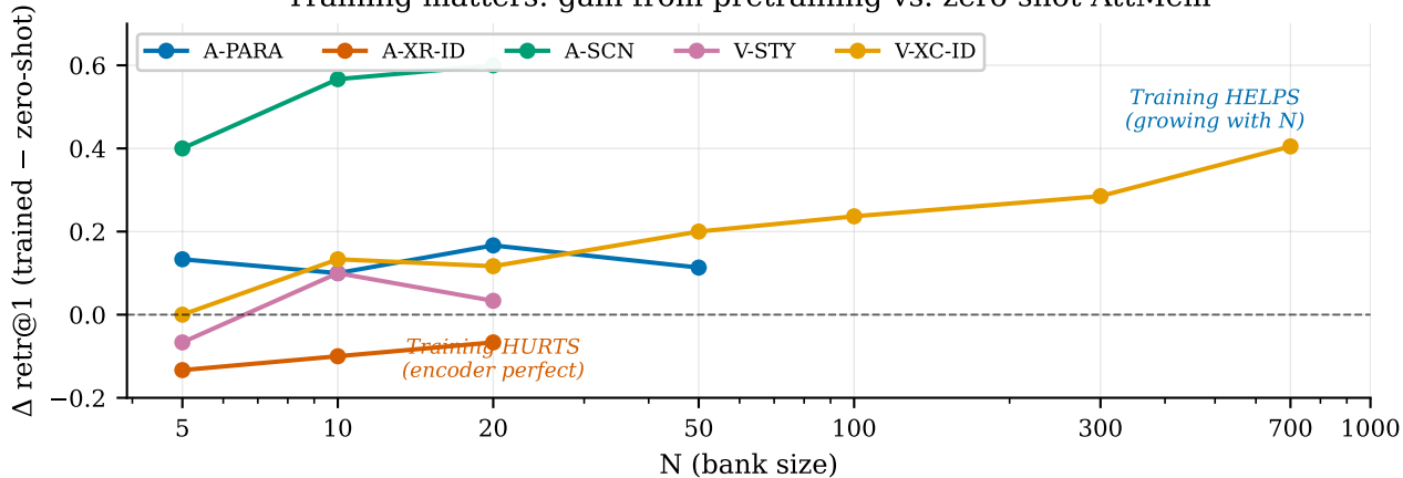
Training matters: gain from pretraining vs. zero-shot AttMem
