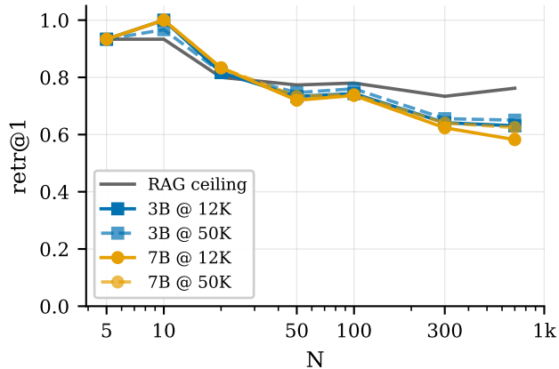
(a) LM size \times training steps
