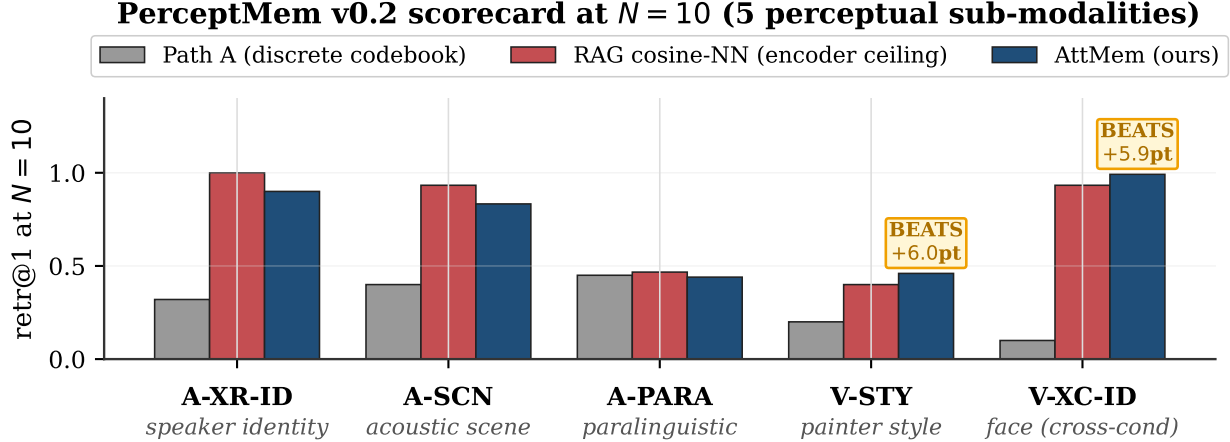
Figure 3: PerceptMem v0.2 scorecard at N=10 . Our parametric multimodal user memory (navy) matches or exceeds the embedding-RAG cosine-NN ceiling on four of five sub-modalities, and exceeds it on V-XC-ID (multi-seed p=0.006 , n=4 ) and V-STY ( p=0.009 , n=5 at N=10 ). The discrete-codebook predecessor (Path A, grey) is 2–10 \times lower across all sub-modalities. BEATS labels show the percentage-point gap over RAG.
