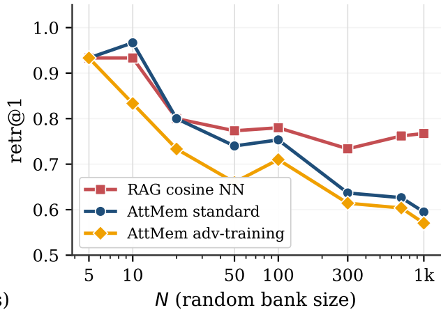
(b) Random regime: trade-off
