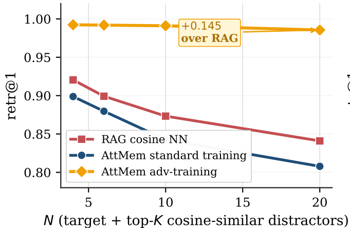
(a) Adversarial regime: training transforms
