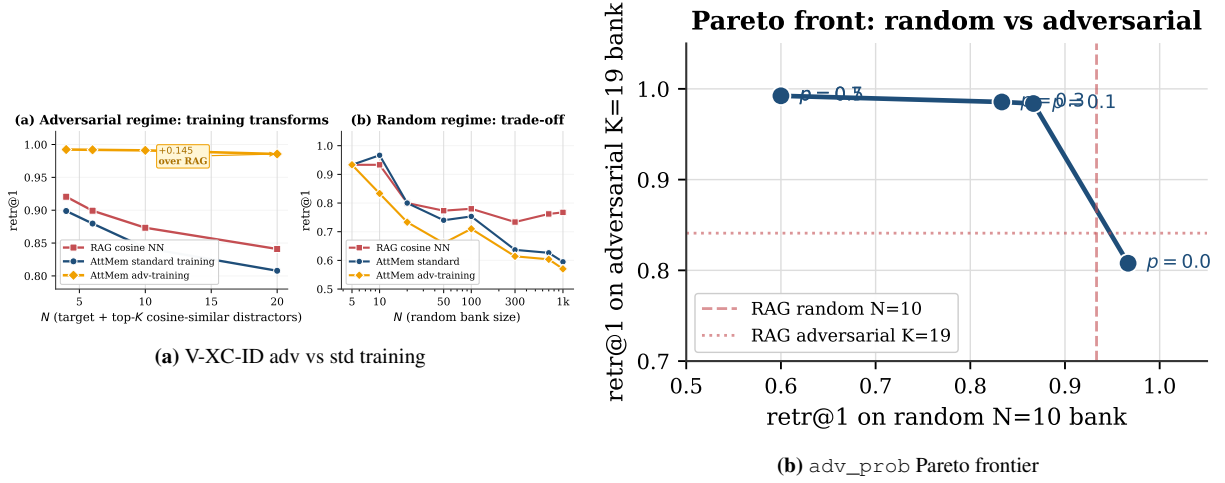
Figure 9: Adv-training mechanics on V-XC-ID-XXXL. Left: standard \rightarrow adv-training transforms the adversarial regime (+14.5pp at K=19 ) at the cost of random-bank retr@1. Right: sweeping adv_prob traces a clean Pareto front; adv_prob \approx 0.1 is the sweet spot — near-best adversarial with minimal random-regime degradation.
