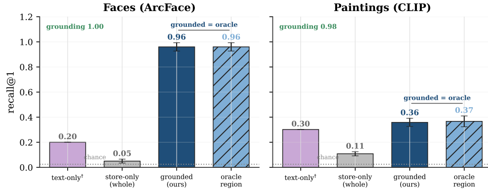
Figure 5. Ablation of the grounded memory on cluttered scenes ( M=40 , two referents per scene). Capability increases left to right: a text-only caption (†, from the matched identity benchmark on clean crops, Figure 4); store-only , embedding the whole scene with no grounding; grounded (ground + identify + store, ours); and the correct-region oracle . Store-only is near chance — below even text-only — while grounding recovers the oracle. Retrieval coincides with store throughout (both are the encoder’s nearest neighbour), so the gain is grounding, not the matcher. Faces: ArcFace, landmark alignment, 5 seeds; paintings: CLIP, no alignment, 3 seeds; error bars \pm 95\% CI.
