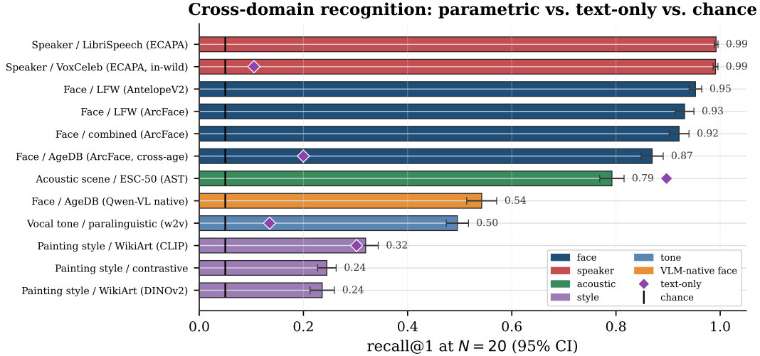
Figure 6. The recognition core across 12 perceptual domains and 5 modalities (1,080 tasks; recall@1 at N=20 , 30 draws, 95% CI), coloured by modality, against chance ( 1/N , black ticks) and the text-only caption baseline where measured (purple diamonds, per modality). Parametric recall tracks the encoder and clears chance everywhere, far exceeding text-only on perceptual identity (speaker, face, tone). The one inversion is the nameable acoustic scene, where a caption (“typing on a keyboard”) edges the weaker AST encoder — exactly the router boundary (§7): text suffices for nameable categories, the parametric bank for identity. The VLM’s own native vision encoder (orange) reads the same AgeDB faces far below a purpose-built one.
