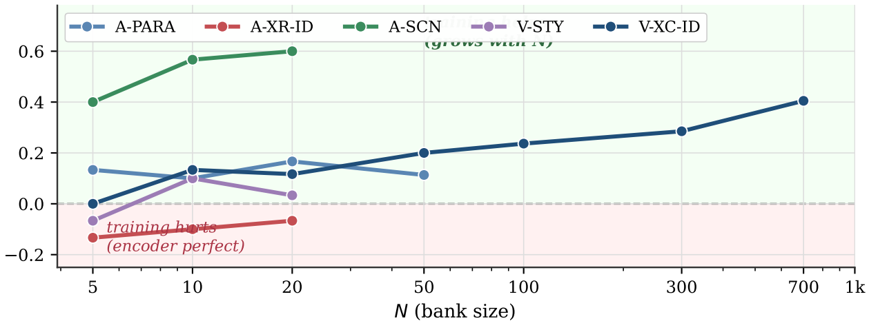
Effect of pretraining: 3 regimes
