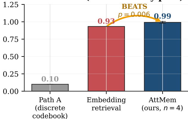
Recall@1 at N=10
