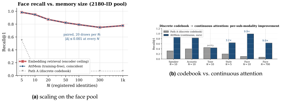
Figure 17. Left: under the paired protocol (20 draws per N ) the training-free read is coincident with the encoder ceiling from N=5 to N=1000 ( |\Delta| \leq 0.001 ; Table 5), both declining gracefully as the pool grows, while the codebook predecessor never gets off the floor. Right: continuous attention beats the discrete codebook 2–10 \times on every sub-modality.
