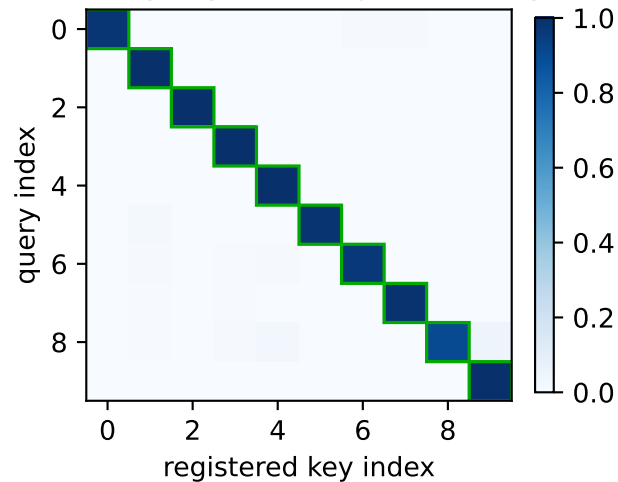
(a) Bank attention weights row=query, col=registered key
