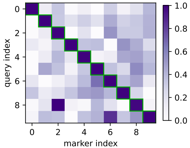
(c) LM marker logits (row-normalised)
