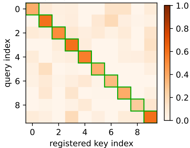
(b) Encoder-cosine similarity row=query, col=registered key
