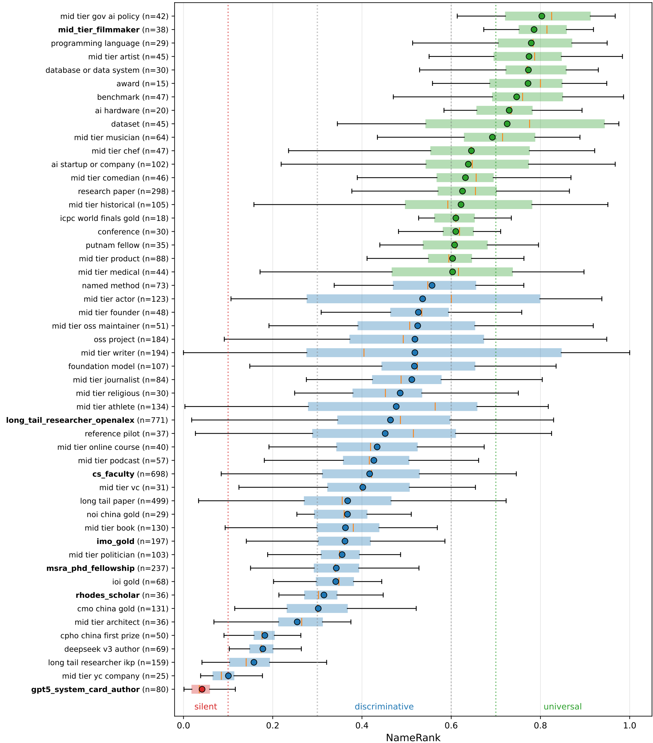
Per-cohort NameRank distribution ( n \geq 10 cohorts) Boxes: IQR; line: median; dot: mean. Three zones visible on a single instrument.
