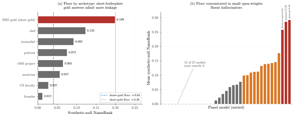
Figure 18: Synthetic-null floor (30 fictional entities through the full pipeline). (a) Floor by archetype: dense-gold cohorts (founder, CS faculty) floor near \sim 0.04 , but the short-boilerplate-gold IMO archetype floors at 0.199 because the generic year+country+medal gold is partly satisfiable from the disambiguating context alone. (b) Per-model synthetic floor: it is concentrated in small open-weights fluent hallucinators (gemma-3-4b at 0.29); 15 of 37 models score the synthetics at exactly 0. The floor sets the noise level below which differences are not evidence of recognition.
