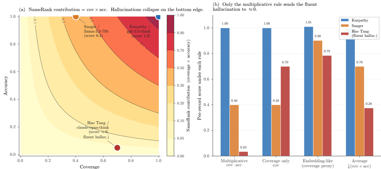
Figure 22: Why the score is multiplicative. (a) The (coverage, accuracy) plane with NameRank = \text{cov} \cdot \text{acc} shown as filled contours. The three appendix worked examples sit at the natural exemplar points: a fully-correct Karpathy bio at (1.0, 1.0), a generic-but-correct Sanger summary at (0.4, 1.0), and the Hao Tang fluent hallucination at (0.7, 0.05). (b) Per-record score under four alternative aggregation rules. Only the multiplicative rule collapses the fluent hallucination to \approx 0 ; coverage-only, embedding-style coverage proxies, and the additive average all credit it at \geq 0.38 .
