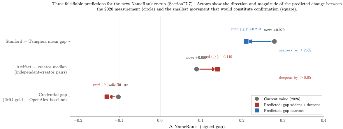
Figure 19: Three falsifiable predictions for the next NameRank re-run. Each row plots a signed gap measured today (circle) and the smallest movement that would constitute confirmation (square). Red arrows mark gaps that widen / deepen under the prediction (credential gap, artifact > creator inversion); blue marks the gap that narrows (corpus-density gradient as Chinese-language training data enters frontier corpora). A re-run on the model fleet released in 2027 will confirm or refute each.
