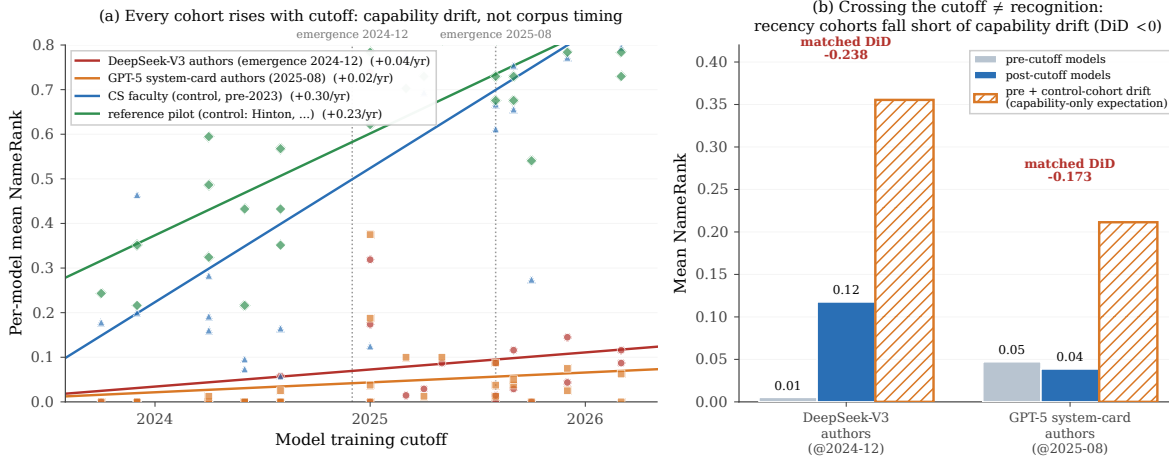
Figure 14. Training-cutoff gradient. (a) Per-model mean NameRank vs. training cutoff for two “recency” cohorts (DeepSeek-V3 authors, GPT-5 system-card authors) and two stable controls; every cohort rises at \sim 0.1\text{--}0.3/\text{yr} , a model-capability confound. (b) The recency cohorts’ pre/post-emergence jump is smaller than the same split on the stable controls, so the matched difference-in-differences is negative ( -0.24 , -0.17 ).
