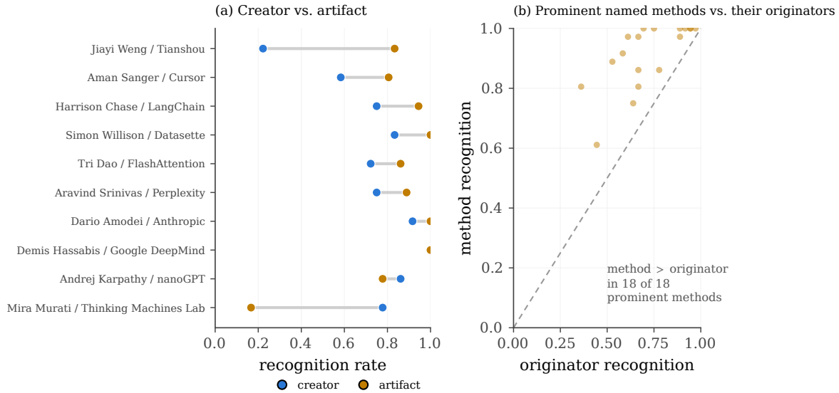
Figure 7. Artifacts usually score higher than their creators. (a) Creator vs. artifact recognition for the 10 resolvable pairs (blue creator, amber artifact), sorted by artifact–creator delta. (b) Named methods vs. their originators.
