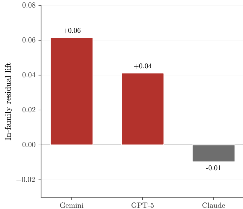
(b) Capability-controlled own-family lift: Gemini/GPT-5 modest, Claude clean
