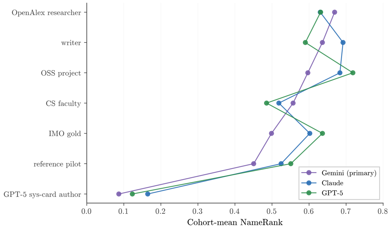
(a) Cohort ladder preserved across judges (pairwise Pearson 0.87--0.93)
