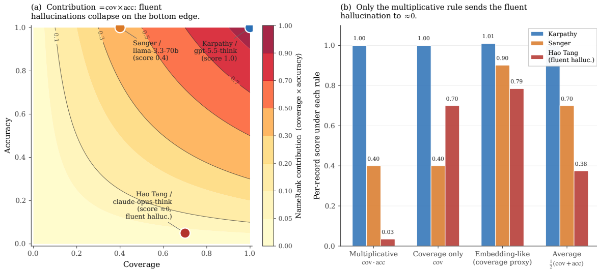
Figure 10. Why the score is multiplicative. (a) The (coverage, accuracy) plane with \text{NameRank} = \text{cov} \cdot \text{acc} shown as filled contours. The three appendix worked examples sit at the natural exemplar points: a fully-correct Karpathy bio at (1.0, 1.0), a generic-but-correct Sanger summary at (0.4, 1.0), and the Hao Tang fluent hallucination at (0.7, 0.05). (b) Per-record score under four alternative aggregation rules. Only the multiplicative rule collapses the fluent hallucination to \approx 0 ; coverage-only, embedding-style coverage proxies, and the additive average all credit it at \geq 0.38 .
