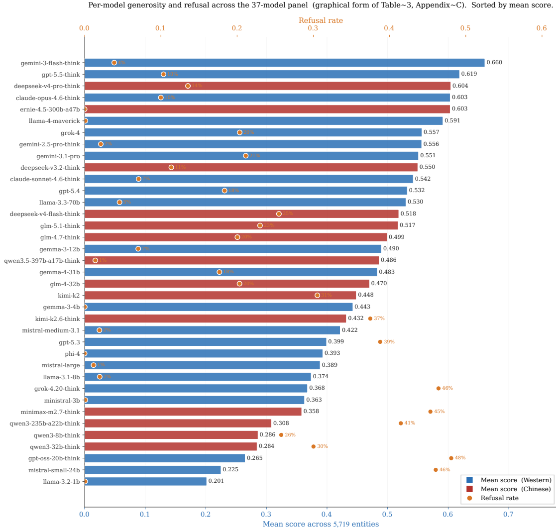
Figure 8. Per-model panel statistics, sorted by mean score (graphical form of Table 15). Bars are mean per-record score across 5,719 entities (lower x-axis, blue/red for Western/Chinese vendor); orange markers on the upper x-axis are the per-model refusal rate, with labels for refusal > 0.001. Two failure regions appear at the row level: the strict cluster at the bottom (gpt-oss-20b-think, mistral-small-24b, qwen3-32b/8b-think) refuses heavily; the fluent-hallucinator cluster (ernie, llama-4-maverick, gemma-3-4b, phi-4, ministral-3b, llama-3.2-1b) shows 0% or near-zero refusal, with widely varying mean scores. The panel mean integrates over both styles.
