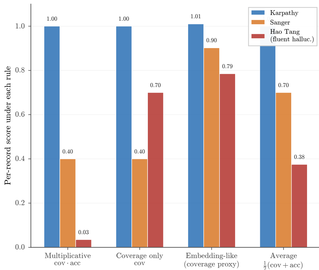
(b) Only the multiplicative rule sends the fluent hallucination to \approx 0 .
