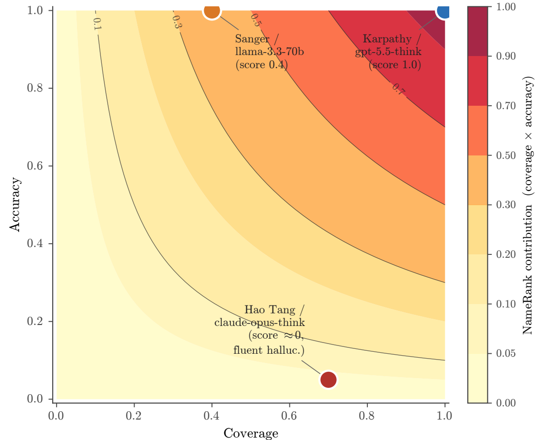
(a) NameRank contribution = \text{cov} \times \text{acc} . Hallucinations collapse on the bottom edge.
